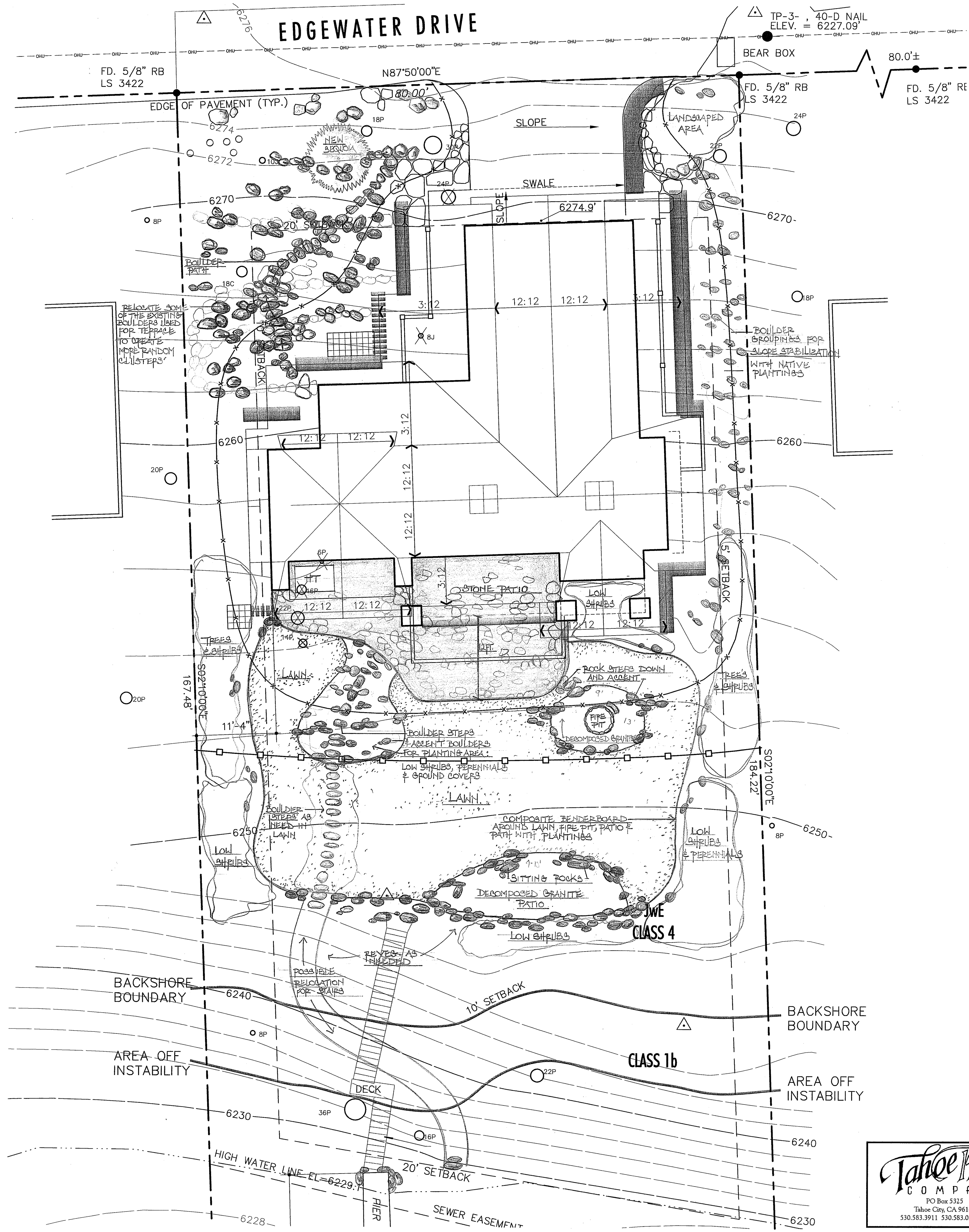
LANDSCAPE PLAN LOT 29 00 04 08 16 feet 093-072-013
